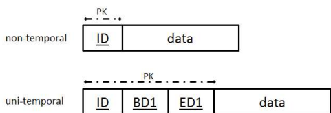
Fig. 2. Uni-temporal model [4]
