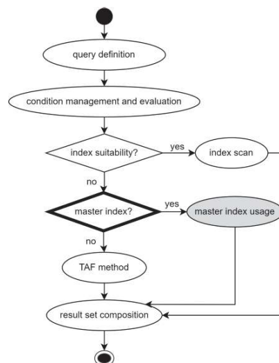
Fig. 6. Data flow - Index access selection [3]
