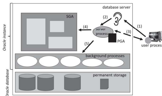
Fig. 1. Database system architecture - user and server process mapping
