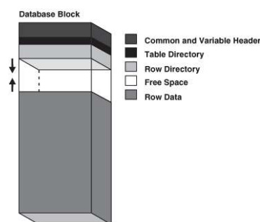
Fig. 5. Database block structure [12]
