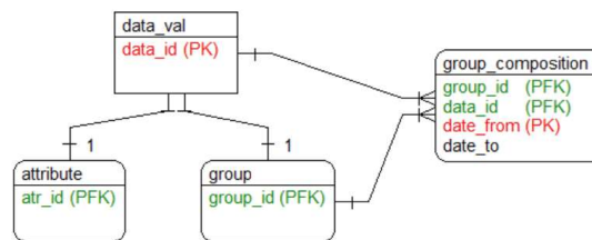
Fig. 4. Data_val composition [5]
